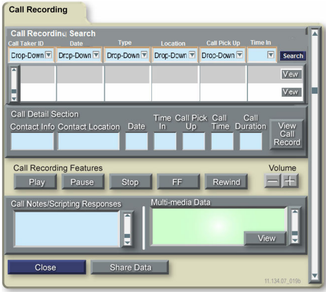
Figure 4.21—Call Recording Pop-Up Screen Layout
